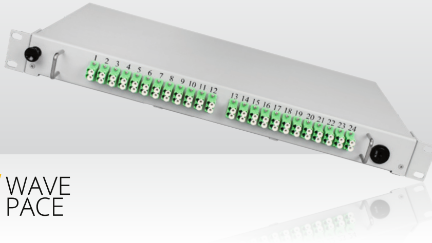
10443957 SP-48-Pull-Panel-LC/APC
