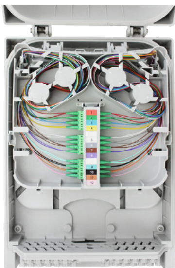
MDU-XL-Wallbox Patch area, pre-installed exemplarily
