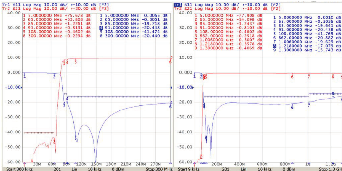
Insertion Loss, Rejection and Return Loss Span: 300/1.300 MHz
