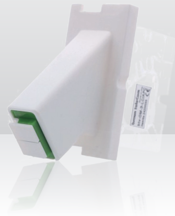
24200050 btv-OM-1-LC/APC, optical click-in module, right slot
